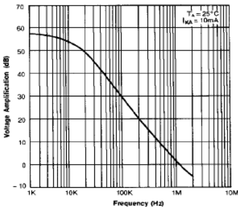
Figure 5. Small Signal Voltage Amplification vs. Frequency
